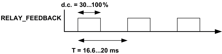
Fig. 5.4: Timing diagram: Signal at input "RELAY_FEEDBACK"
