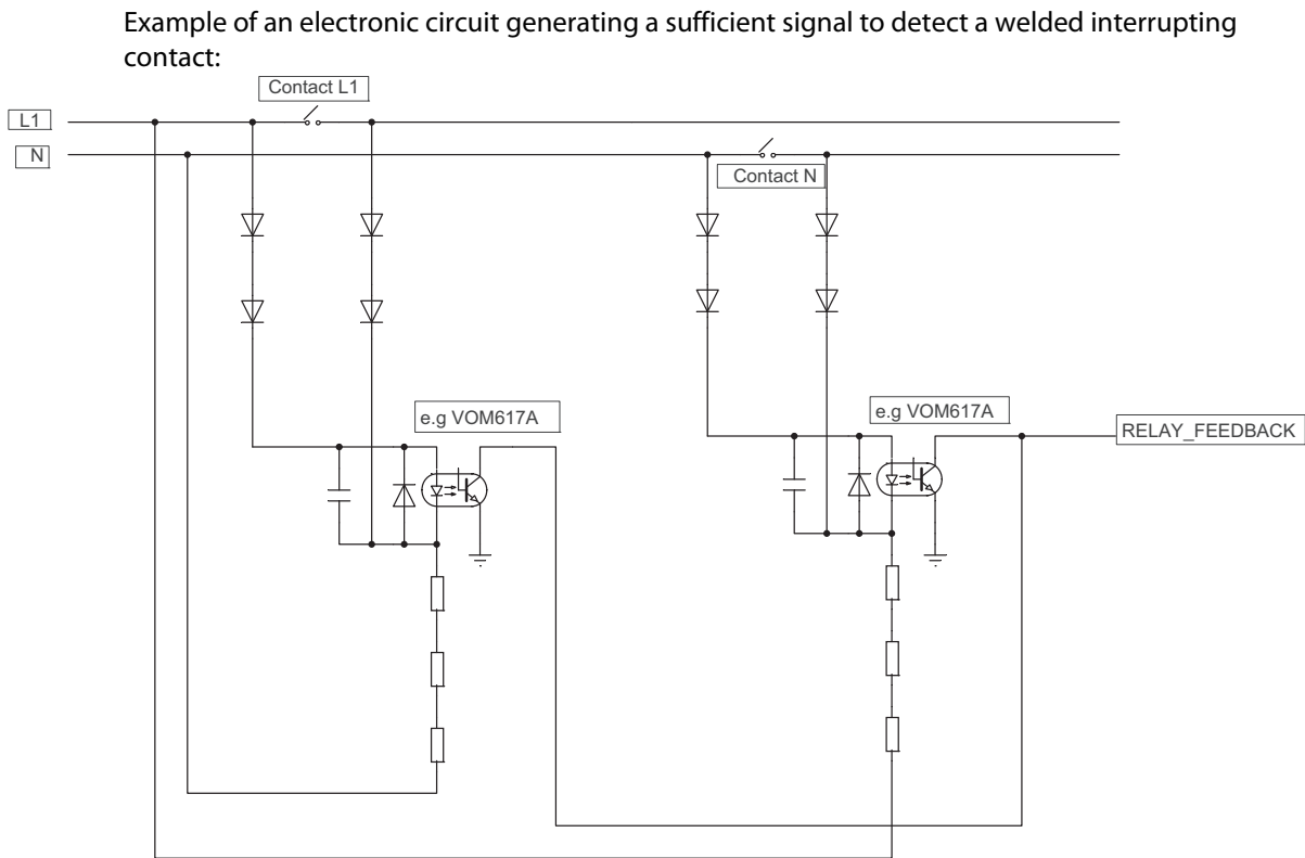
Fig. 5.3: Wiring diagram
