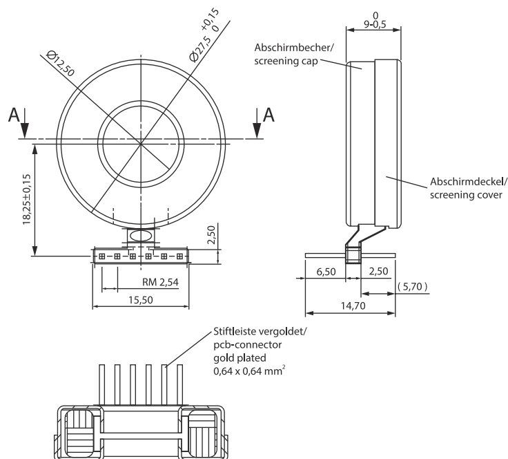
Fig. 6.5: WN12-01 (dimensions in mm)
