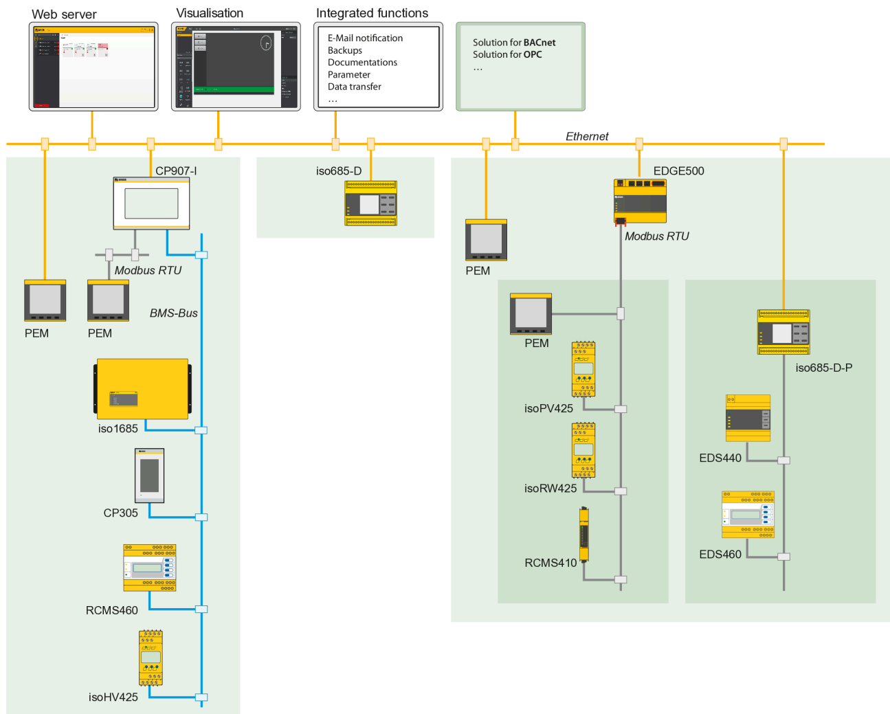
Block diagram
