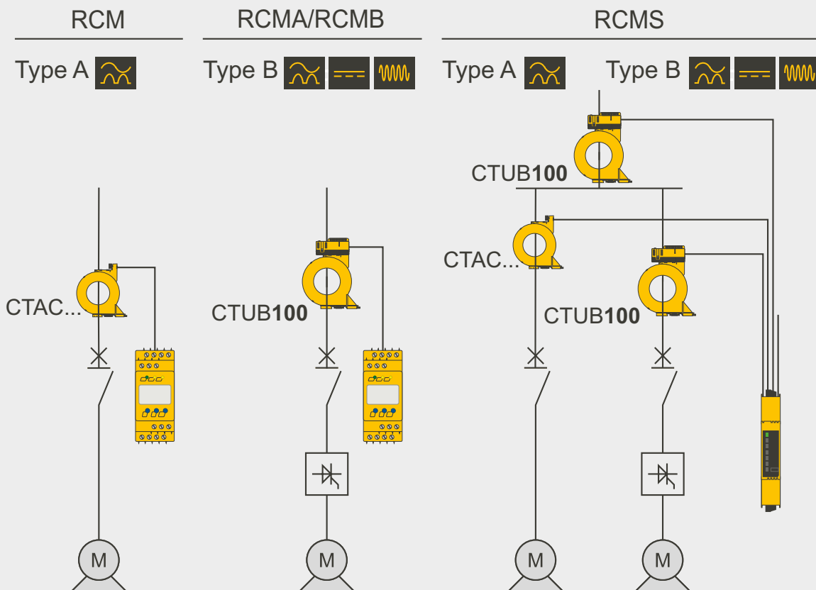
RCM/RCMA/RCMB/RCMS application
